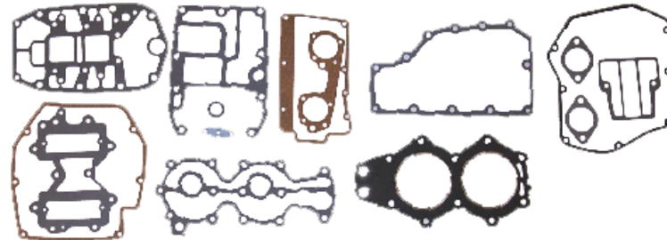
18-4305 AP# 13282 POWERHEAD GASKET SET Replaces: 393433
